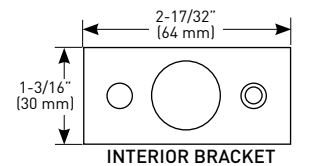
INTERIOR BRACKET
